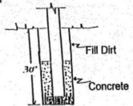
DETAIL C
